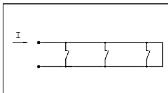
Figure 4, Parallel connection
