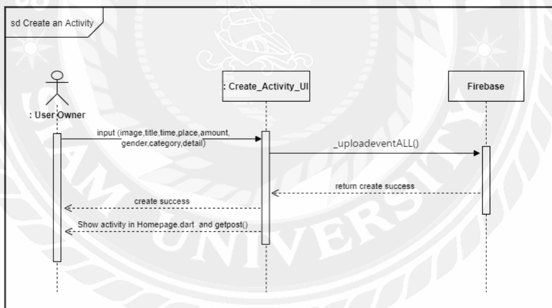
រូបភាព 3.5 Sequence diagram : Create an Activity
